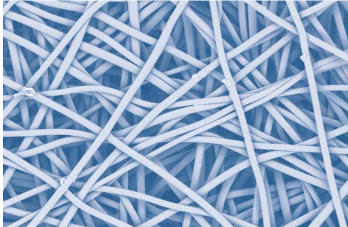
SEM picture of a high-performance filter medium
